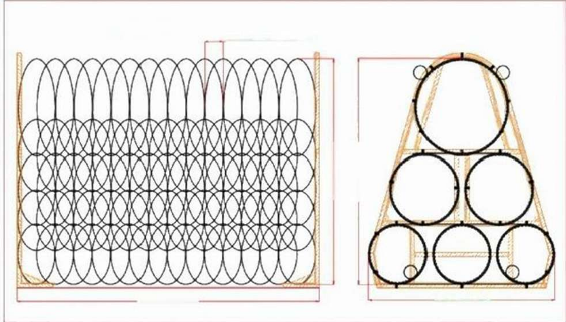
6D razor wire trailer
